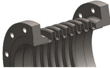
Style 55 (Fixed 150# RFSO Flanges) SHP series have 300# RFSO Flanges
